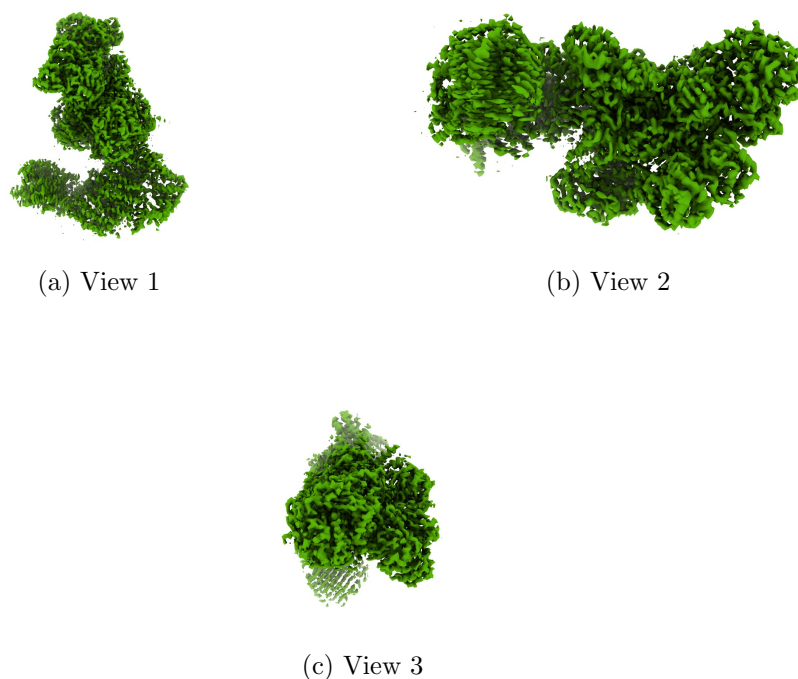
Figure 4: Isosurface at threshold=0.028500. Views generated by ChimeraX at a the following X, Y, Z angles: View 1 (0, -90, -90), View 2 (-90, 0, -90), View 3 (0, 0, 0).
