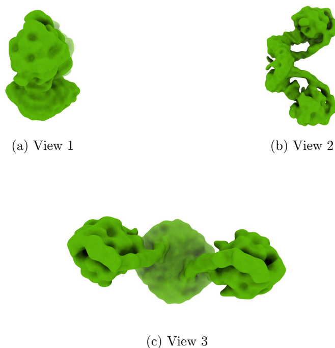
Figure 4: Isosurface at threshold=0.007720. Views generated by ChimeraX at a the following X, Y, Z angles: View 1 (0, -90, -90), View 2 (-90, 0, -90), View 3 (0, 0, 0).
