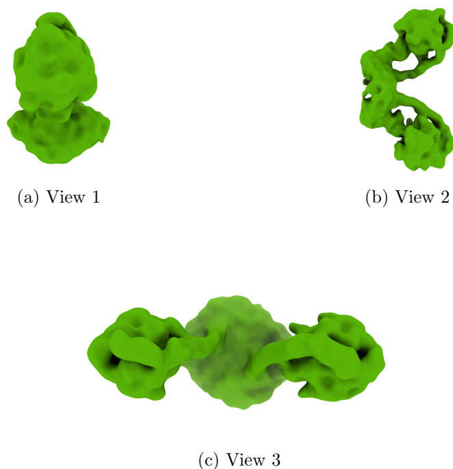
Figure 4: Isosurface at threshold=0.007170. Views generated by ChimeraX at a the following X, Y, Z angles: View 1 (0, -90, -90), View 2 (-90, 0, -90), View 3 (0, 0, 0).
