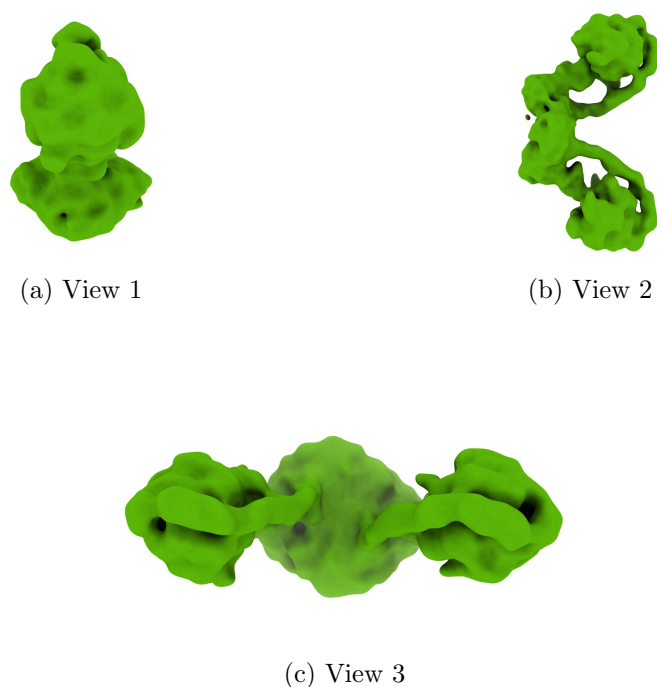
Figure 4: Isosurface at threshold=0.008120. Views generated by ChimeraX at a the following X, Y, Z angles: View 1 (0, -90, -90), View 2 (-90, 0, -90), View 3 (0, 0, 0).
