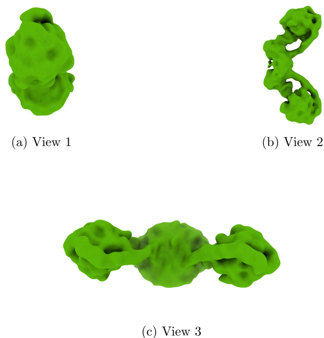
Figure 4: Isosurface at threshold=0.006670. Views generated by ChimeraX at a the following X, Y, Z angles: View 1 (0, -90, -90), View 2 (-90, 0, -90), View 3 (0, 0, 0).
