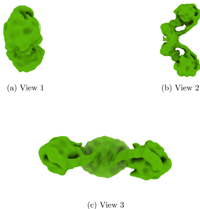
Figure 4: Isosurface at threshold=0.006420. Views generated by ChimeraX at a the following X, Y, Z angles: View 1 (0, -90, -90), View 2 (-90, 0, -90), View 3 (0, 0, 0).
