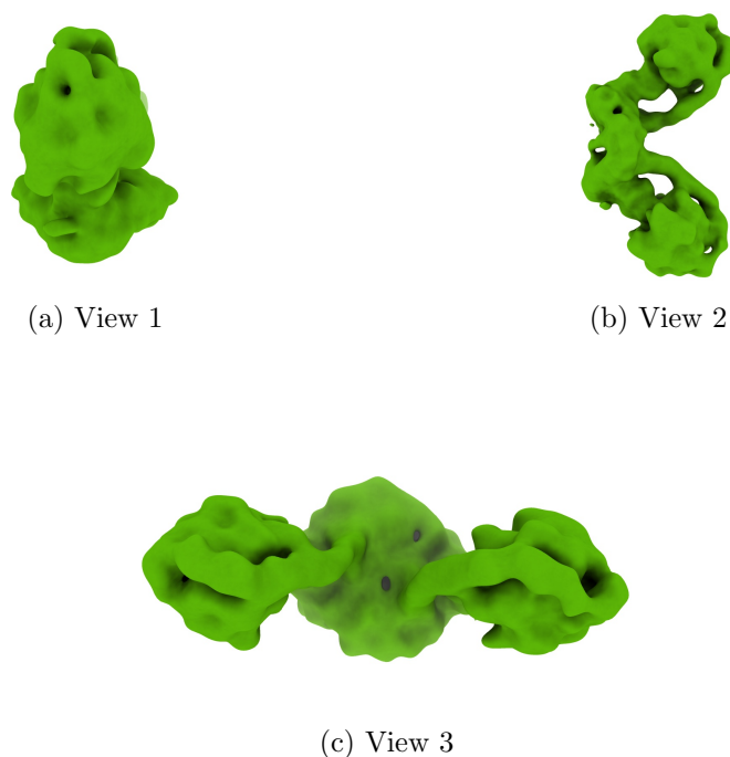
Figure 4: Isosurface at threshold=0.007090. Views generated by ChimeraX at a the following X, Y, Z angles: View 1 (0, -90, -90), View 2 (-90, 0, -90), View 3 (0, 0, 0).
