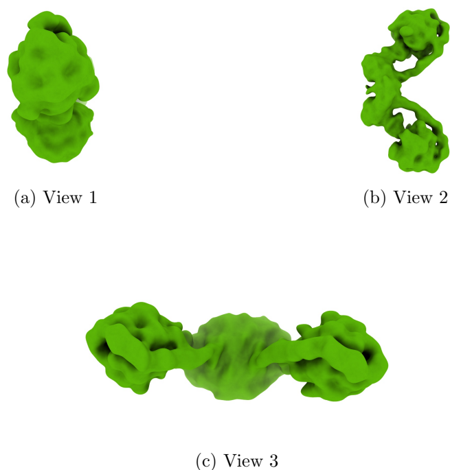
Figure 4: Isosurface at threshold=0.007710. Views generated by ChimeraX at a the following X, Y, Z angles: View 1 (0, -90, -90), View 2 (-90, 0, -90), View 3 (0, 0, 0).
