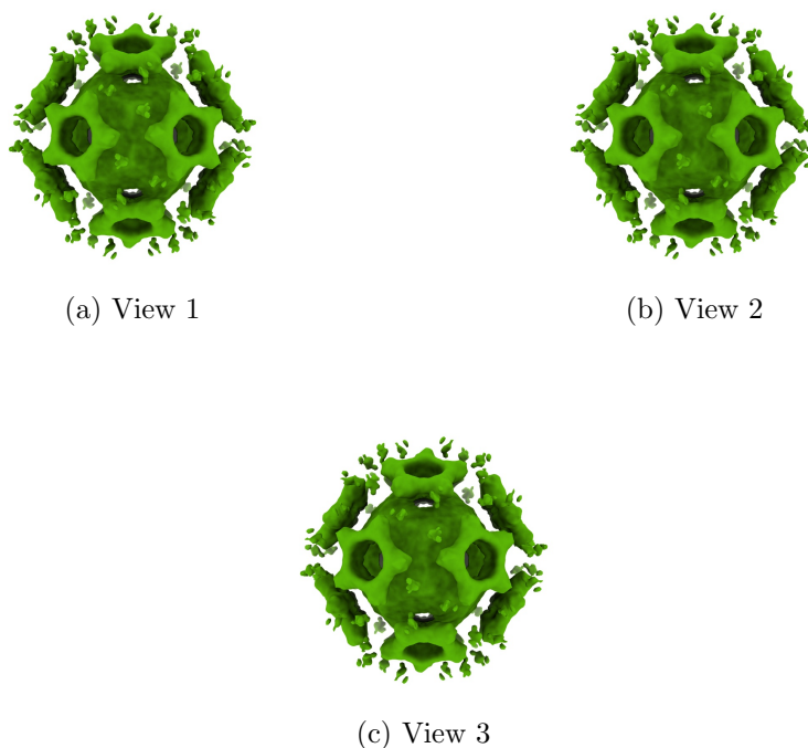
Figure 4: Isosurface at threshold=47.400000. Views generated by ChimeraX at a the following X, Y, Z angles: View 1 (0, -90, -90), View 2 (-90, 0, -90), View 3 (0, 0, 0).
