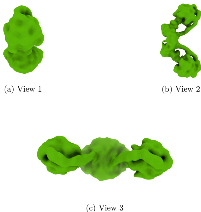
Figure 4: Isosurface at threshold=0.006870. Views generated by ChimeraX at a the following X, Y, Z angles: View 1 (0, -90, -90), View 2 (-90, 0, -90), View 3 (0, 0, 0).
