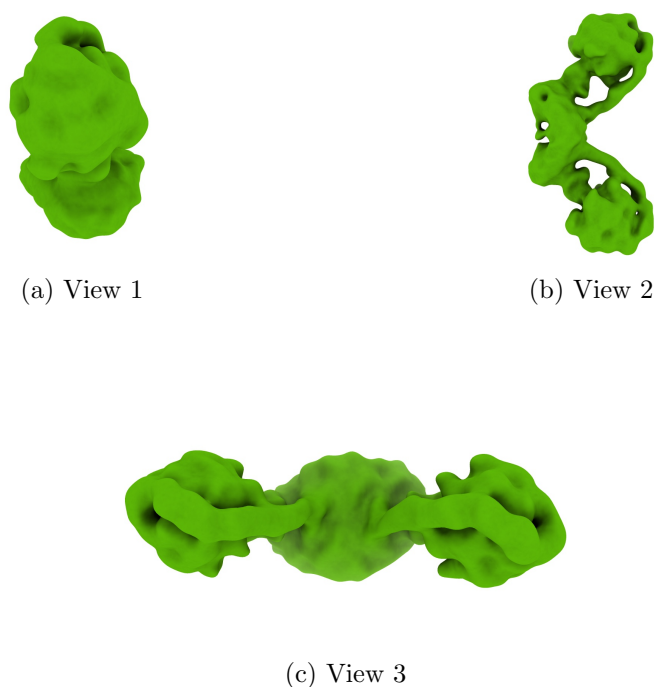
Figure 4: Isosurface at threshold=0.007020. Views generated by ChimeraX at a the following X, Y, Z angles: View 1 (0, -90, -90), View 2 (-90, 0, -90), View 3 (0, 0, 0).
