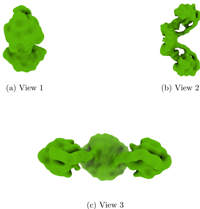
Figure 4: Isosurface at threshold=0.006380. Views generated by ChimeraX at a the following X, Y, Z angles: View 1 (0, -90, -90), View 2 (-90, 0, -90), View 3 (0, 0, 0).
