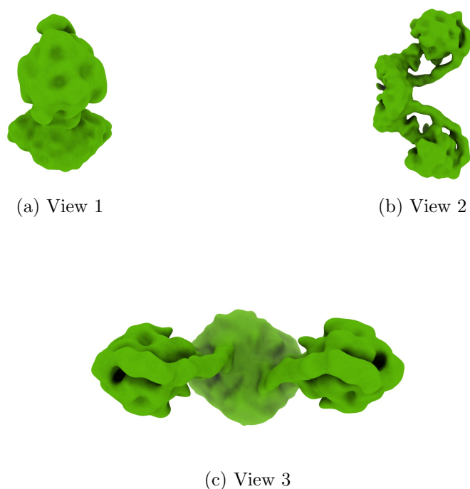
Figure 4: Isosurface at threshold=0.007690. Views generated by ChimeraX at a the following X, Y, Z angles: View 1 (0, -90, -90), View 2 (-90, 0, -90), View 3 (0, 0, 0).
