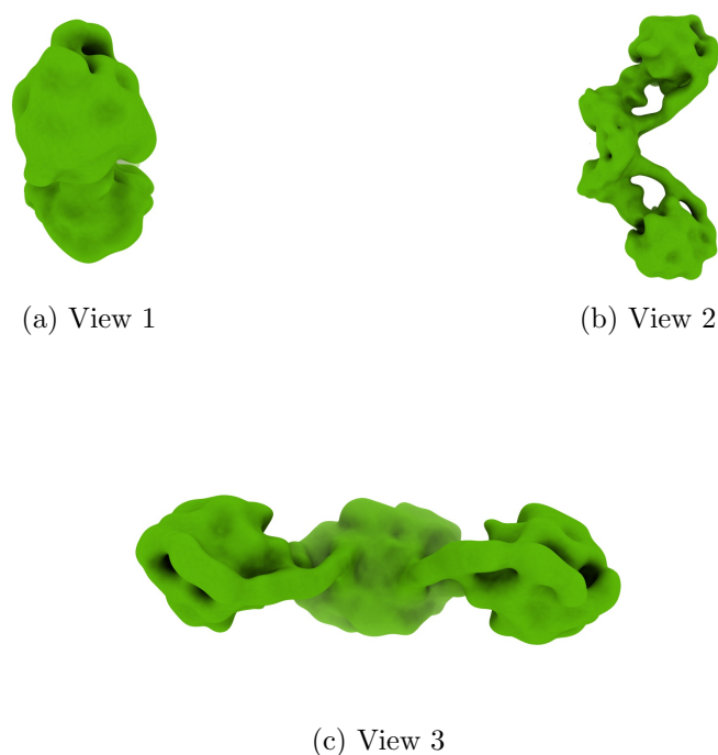
Figure 4: Isosurface at threshold=0.008020. Views generated by ChimeraX at a the following X, Y, Z angles: View 1 (0, -90, -90), View 2 (-90, 0, -90), View 3 (0, 0, 0).
