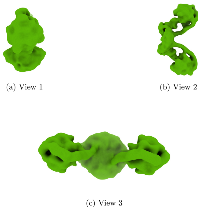
Figure 4: Isosurface at threshold=0.007510. Views generated by ChimeraX at a the following X, Y, Z angles: View 1 (0, -90, -90), View 2 (-90, 0, -90), View 3 (0, 0, 0).
