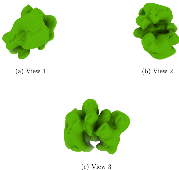
Figure 4: Isosurface at threshold=0.050300. Views generated by ChimeraX at a the following X, Y, Z angles: View 1 (0, -90, -90), View 2 (-90, 0, -90), View 3 (0, 0, 0).
