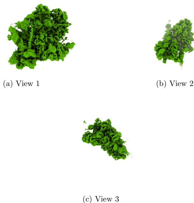
Figure 4: Isosurface at threshold=0.045000. Views generated by ChimeraX at a the following X, Y, Z angles: View 1 (0, -90, -90), View 2 (-90, 0, -90), View 3 (0, 0, 0).
