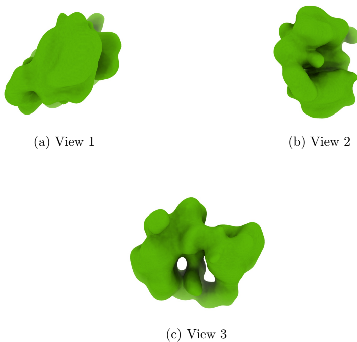
Figure 4: Isosurface at threshold=0.359000. Views generated by ChimeraX at a the following X, Y, Z angles: View 1 (0, -90, -90), View 2 (-90, 0, -90), View 3 (0, 0, 0).
