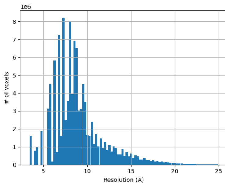
Figure 24: Histogram of the local resolution according to MonoRes.
