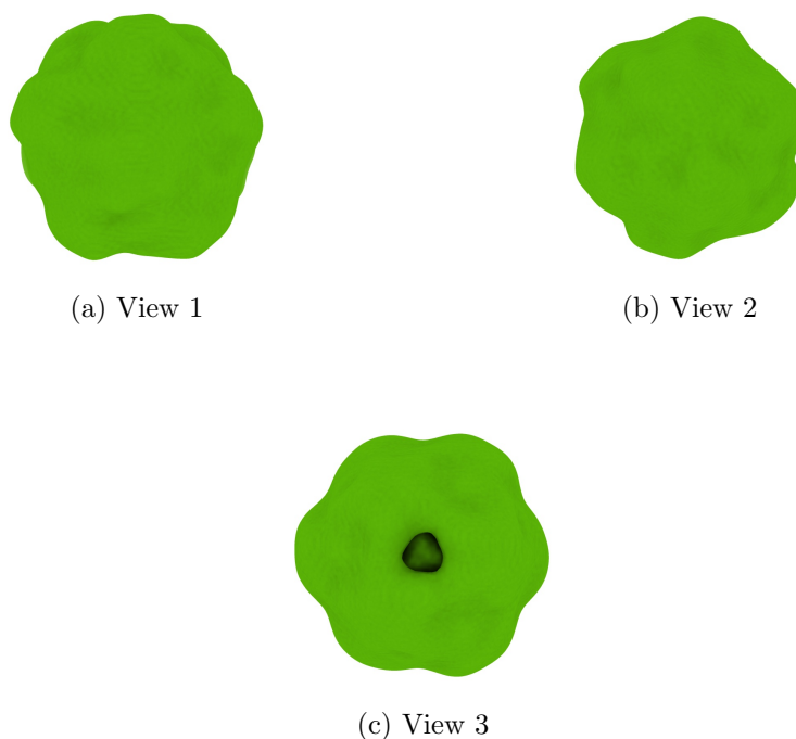
Figure 4: Isosurface at threshold=0.098300. Views generated by ChimeraX at a the following X, Y, Z angles: View 1 (0, -90, -90), View 2 (-90, 0, -90), View 3 (0, 0, 0).
