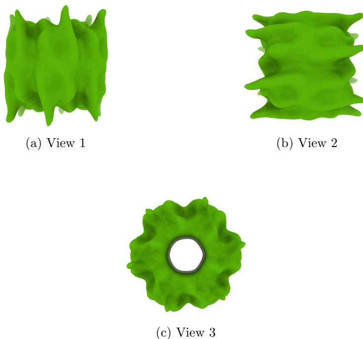
Figure 4: Isosurface at threshold=0.802000. Views generated by ChimeraX at a the following X, Y, Z angles: View 1 (0, -90, -90), View 2 (-90, 0, -90), View 3 (0, 0, 0).
