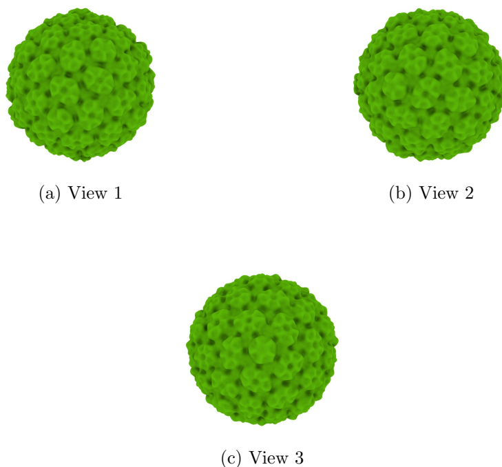
Figure 4: Isosurface at threshold=0.315000. Views generated by ChimeraX at a the following X, Y, Z angles: View 1 (0, -90, -90), View 2 (-90, 0, -90), View 3 (0, 0, 0).
