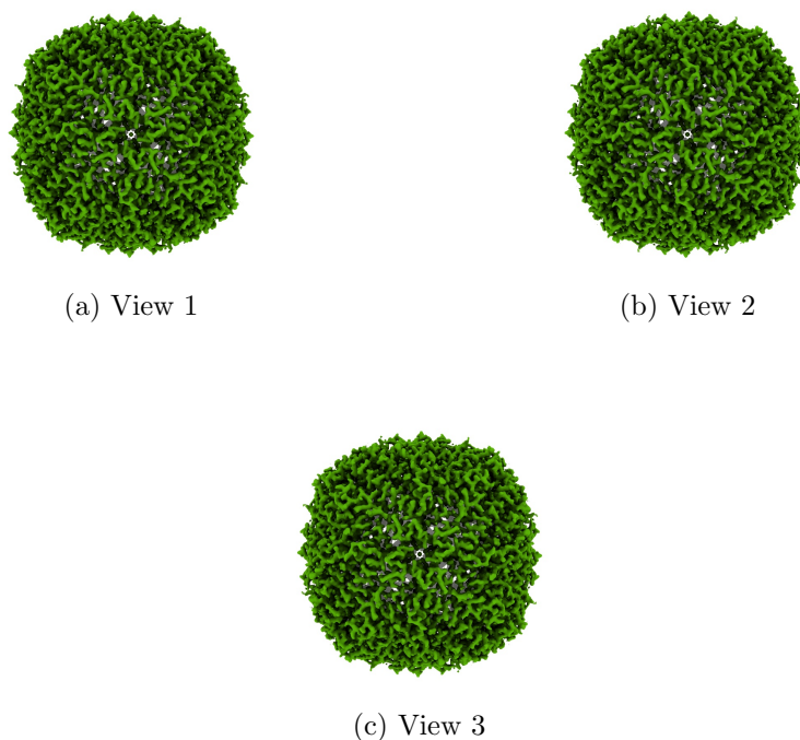
Figure 4: Isosurface at threshold=0.000119. Views generated by ChimeraX at a the following X, Y, Z angles: View 1 (0, -90, -90), View 2 (-90, 0, -90), View 3 (0, 0, 0).
