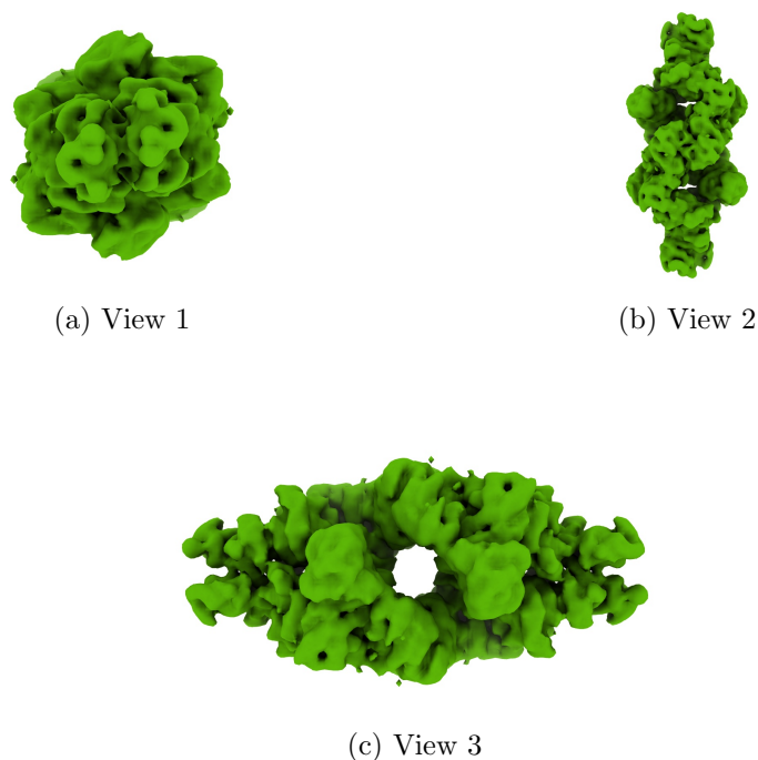
Figure 4: Isosurface at threshold=0.007600. Views generated by ChimeraX at a the following X, Y, Z angles: View 1 (0, -90, -90), View 2 (-90, 0, -90), View 3 (0, 0, 0).
