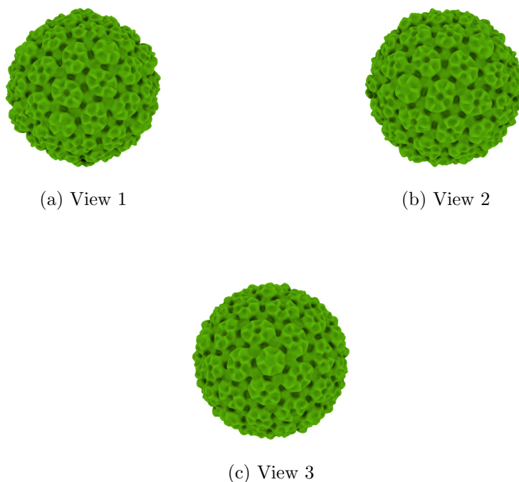
Figure 4: Isosurface at threshold=0.321000. Views generated by ChimeraX at a the following X, Y, Z angles: View 1 (0, -90, -90), View 2 (-90, 0, -90), View 3 (0, 0, 0).
