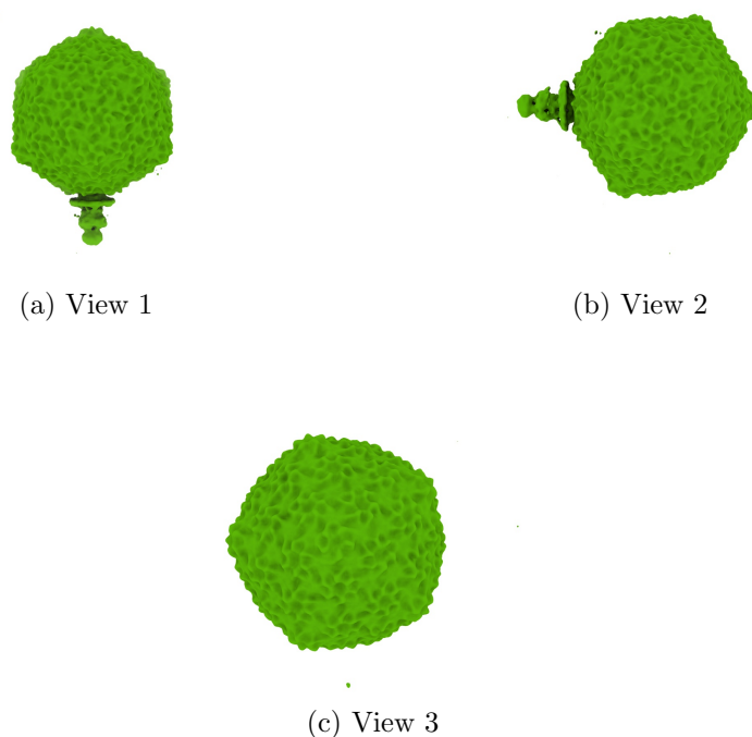
Figure 4: Isosurface at threshold=0.186000. Views generated by ChimeraX at a the following X, Y, Z angles: View 1 (0, -90, -90), View 2 (-90, 0, -90), View 3 (0, 0, 0).
