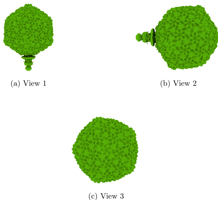
Figure 4: Isosurface at threshold=0.187000. Views generated by ChimeraX at a the following X, Y, Z angles: View 1 (0, -90, -90), View 2 (-90, 0, -90), View 3 (0, 0, 0).
