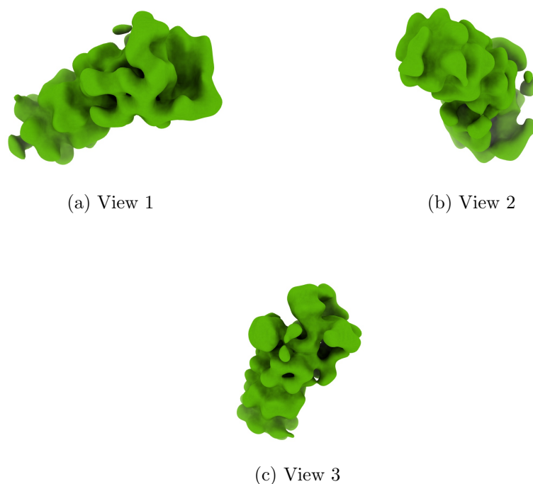
Figure 4: Isosurface at threshold=0.002900. Views generated by ChimeraX at a the following X, Y, Z angles: View 1 (0, -90, -90), View 2 (-90, 0, -90), View 3 (0, 0, 0).
