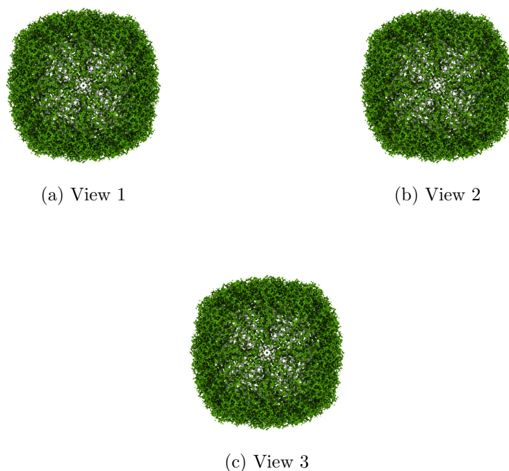
Figure 4: Isosurface at threshold=0.001480. Views generated by ChimeraX at a the following X, Y, Z angles: View 1 (0, -90, -90), View 2 (-90, 0, -90), View 3 (0, 0, 0).
