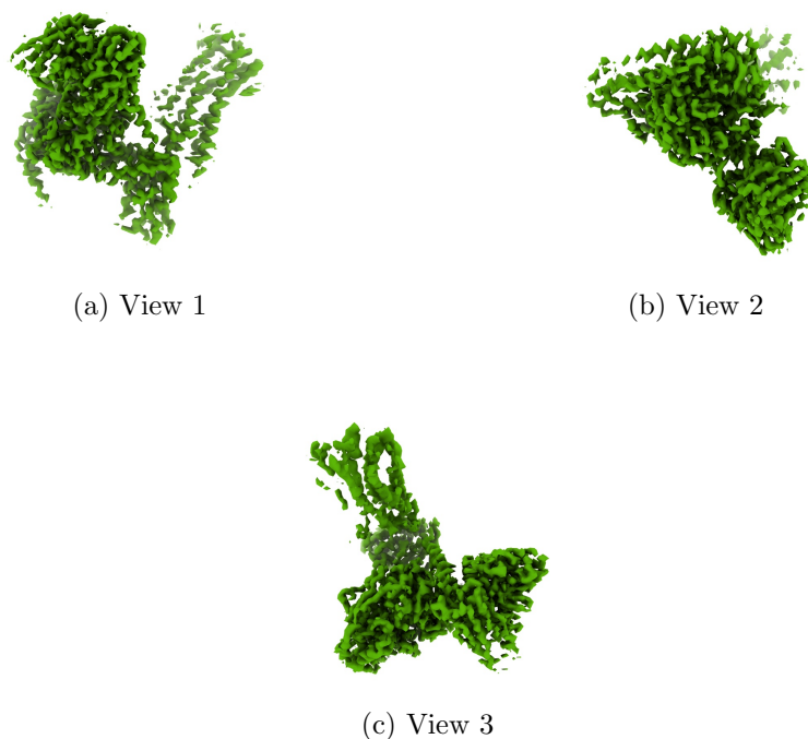
Figure 4: Isosurface at threshold=0.000095. Views generated by ChimeraX at a the following X, Y, Z angles: View 1 (0, -90, -90), View 2 (-90, 0, -90), View 3 (0, 0, 0).
