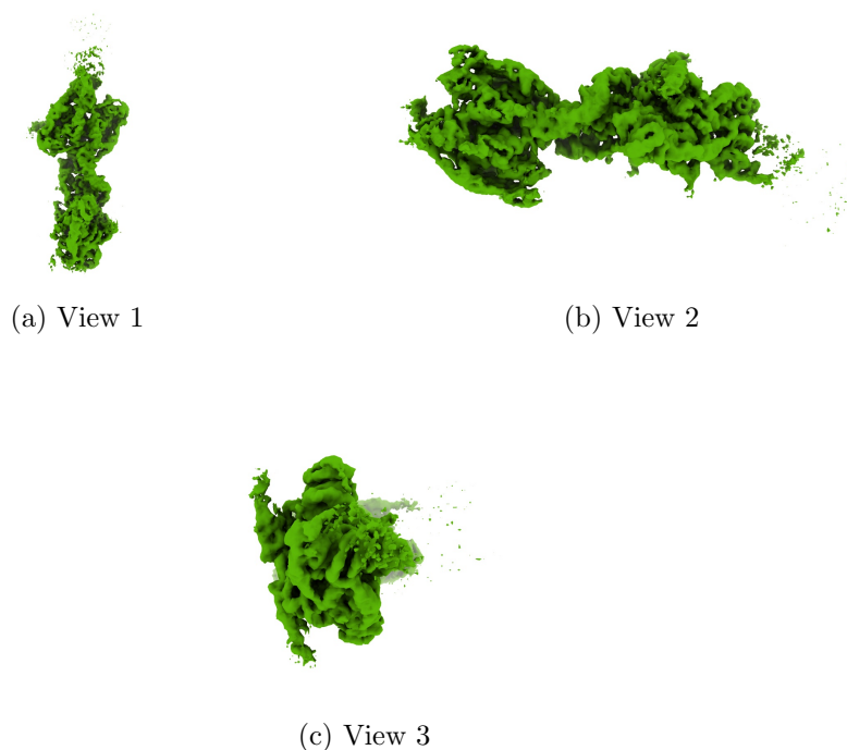
Figure 4: Isosurface at threshold=0.099000. Views generated by ChimeraX at a the following X, Y, Z angles: View 1 (0, -90, -90), View 2 (-90, 0, -90), View 3 (0, 0, 0).
