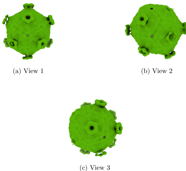
Figure 4: Isosurface at threshold=0.012100. Views generated by ChimeraX at a the following X, Y, Z angles: View 1 (0, -90, -90), View 2 (-90, 0, -90), View 3 (0, 0, 0).
