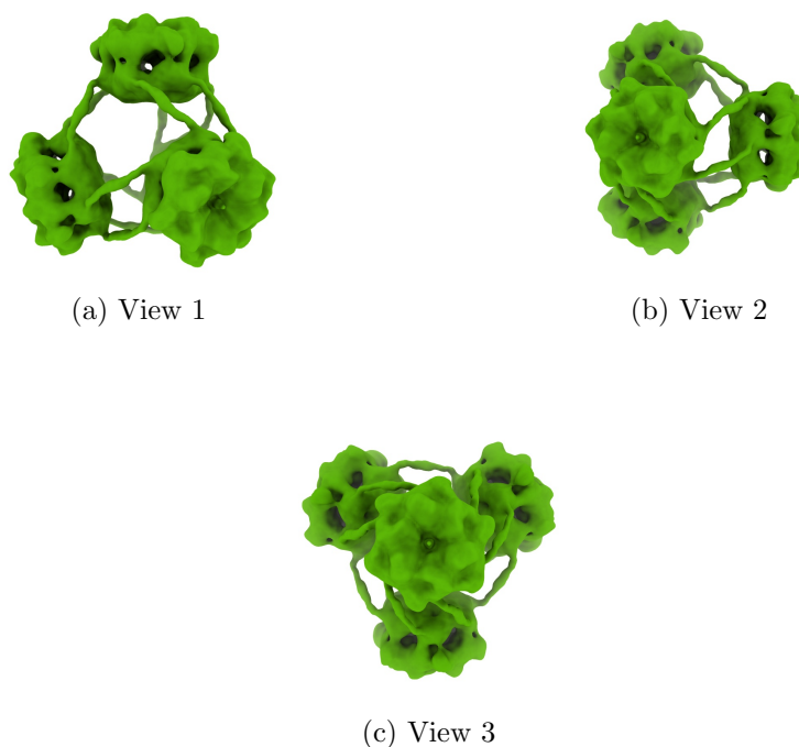
Figure 4: Isosurface at threshold=0.360000. Views generated by ChimeraX at a the following X, Y, Z angles: View 1 (0, -90, -90), View 2 (-90, 0, -90), View 3 (0, 0, 0).
