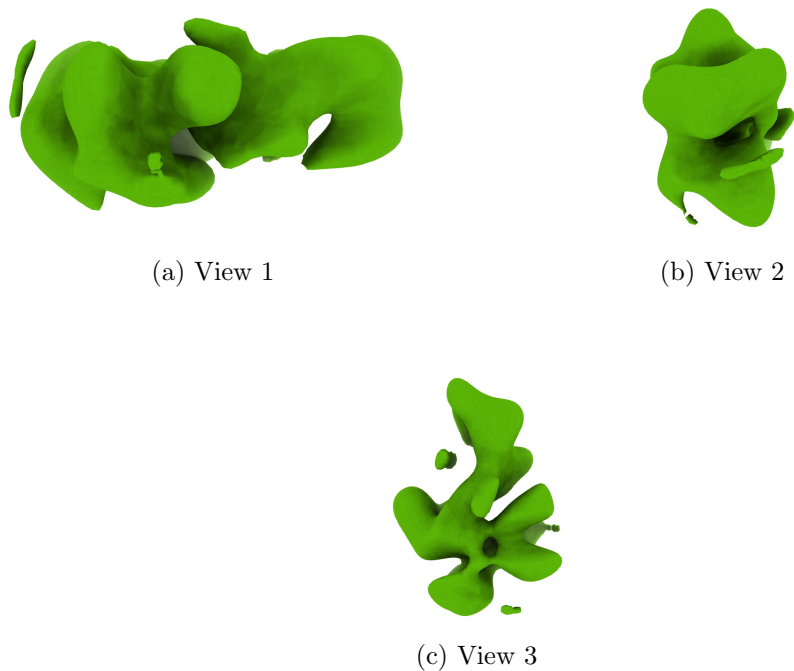
Figure 4: Isosurface at threshold=0.052900. Views generated by ChimeraX at a the following X, Y, Z angles: View 1 (0, -90, -90), View 2 (-90, 0, -90), View 3 (0, 0, 0).
