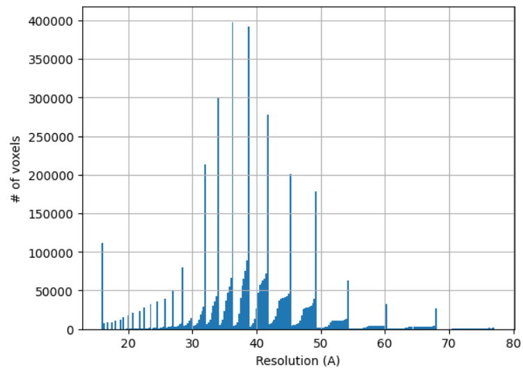
Figure 23: Histogram of the local resolution according to MonoRes.
