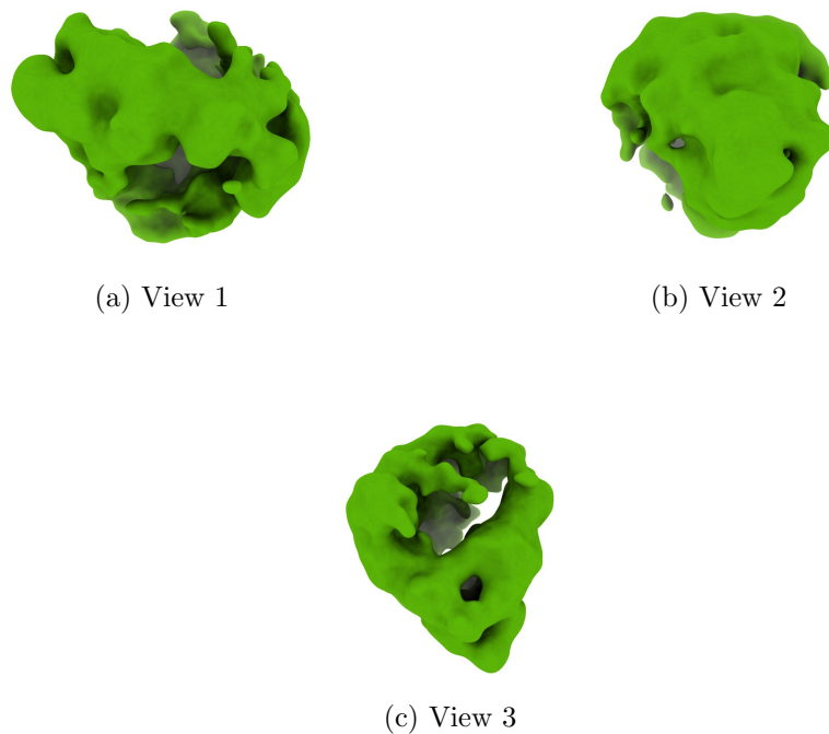
Figure 4: Isosurface at threshold=0.697000. Views generated by ChimeraX at a the following X, Y, Z angles: View 1 (0, -90, -90), View 2 (-90, 0, -90), View 3 (0, 0, 0).
