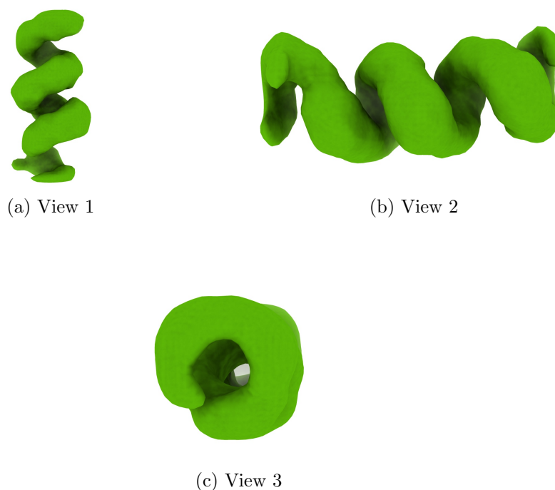
Figure 4: Isosurface at threshold=0.070900. Views generated by ChimeraX at a the following X, Y, Z angles: View 1 (0, -90, -90), View 2 (-90, 0, -90), View 3 (0, 0, 0).
