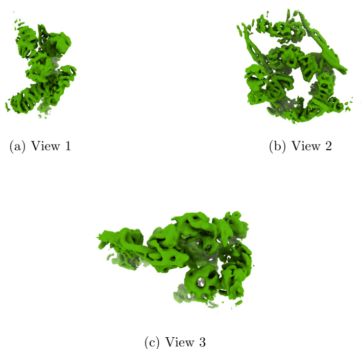
Figure 4: Isosurface at threshold=0.028800. Views generated by ChimeraX at a the following X, Y, Z angles: View 1 (0, -90, -90), View 2 (-90, 0, -90), View 3 (0, 0, 0).
