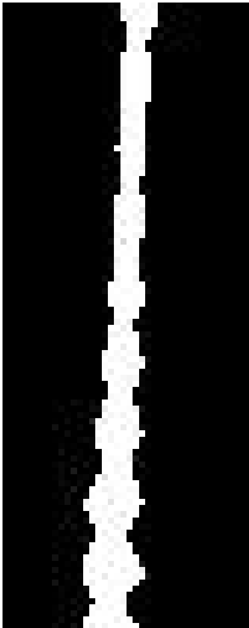
(a) X Slice 18
