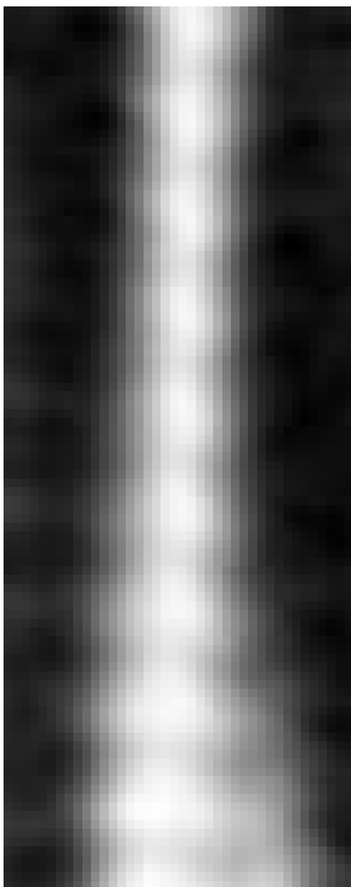
(a) X Slice 19
