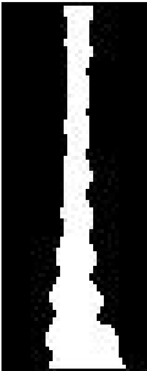
(a) X Slice 20
