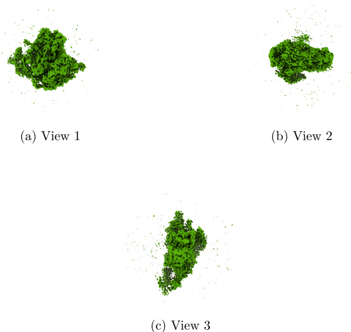
Figure 4: Isosurface at threshold=0.026400. Views generated by ChimeraX at a the following X, Y, Z angles: View 1 (0, -90, -90), View 2 (-90, 0, -90), View 3 (0, 0, 0).
