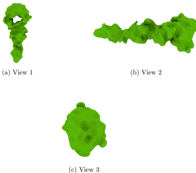
Figure 4: Isosurface at threshold=0.003230. Views generated by ChimeraX at a the following X, Y, Z angles: View 1 (0, -90, -90), View 2 (-90, 0, -90), View 3 (0, 0, 0).
