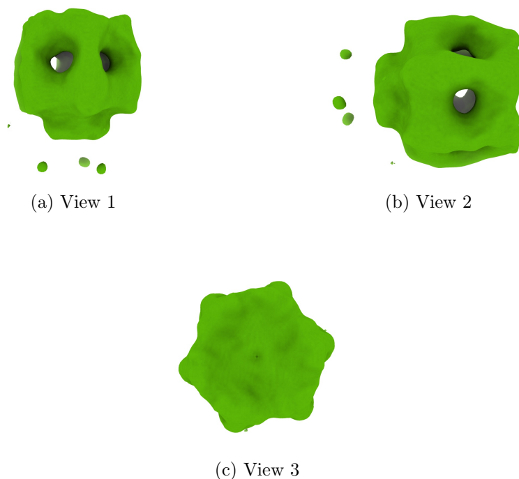
Figure 4: Isosurface at threshold=0.356000. Views generated by ChimeraX at a the following X, Y, Z angles: View 1 (0, -90, -90), View 2 (-90, 0, -90), View 3 (0, 0, 0).
