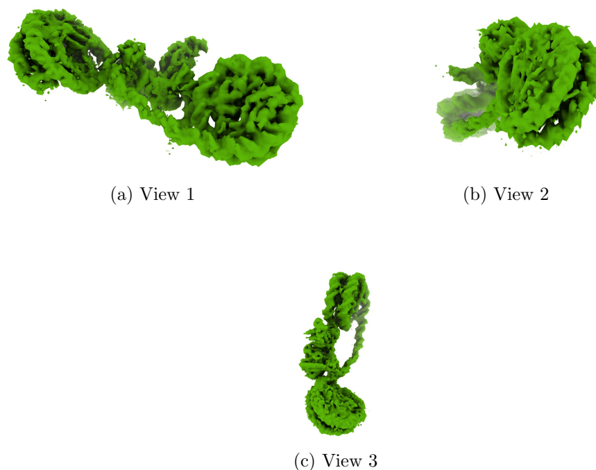
Figure 4: Isosurface at threshold=0.026300. Views generated by ChimeraX at a the following X, Y, Z angles: View 1 (0, -90, -90), View 2 (-90, 0, -90), View 3 (0, 0, 0).
