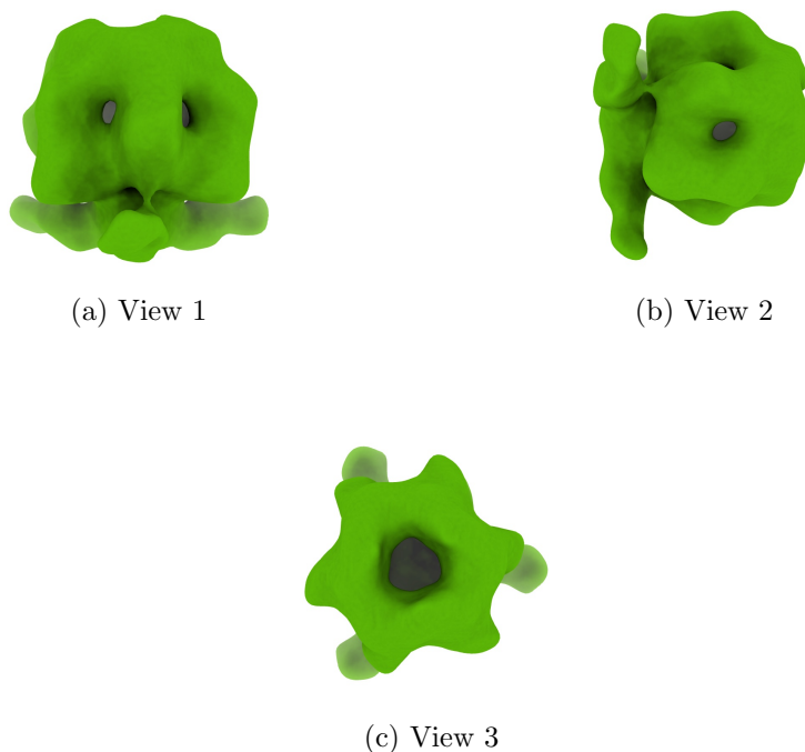
Figure 4: Isosurface at threshold=0.052100. Views generated by ChimeraX at a the following X, Y, Z angles: View 1 (0, -90, -90), View 2 (-90, 0, -90), View 3 (0, 0, 0).
