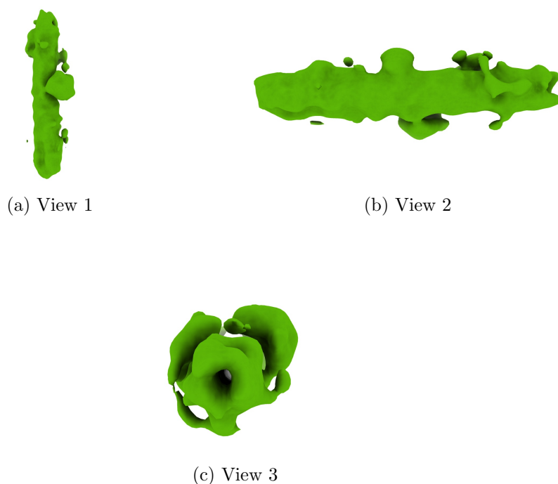
Figure 4: Isosurface at threshold=2.300000. Views generated by ChimeraX at a the following X, Y, Z angles: View 1 (0, -90, -90), View 2 (-90, 0, -90), View 3 (0, 0, 0).
