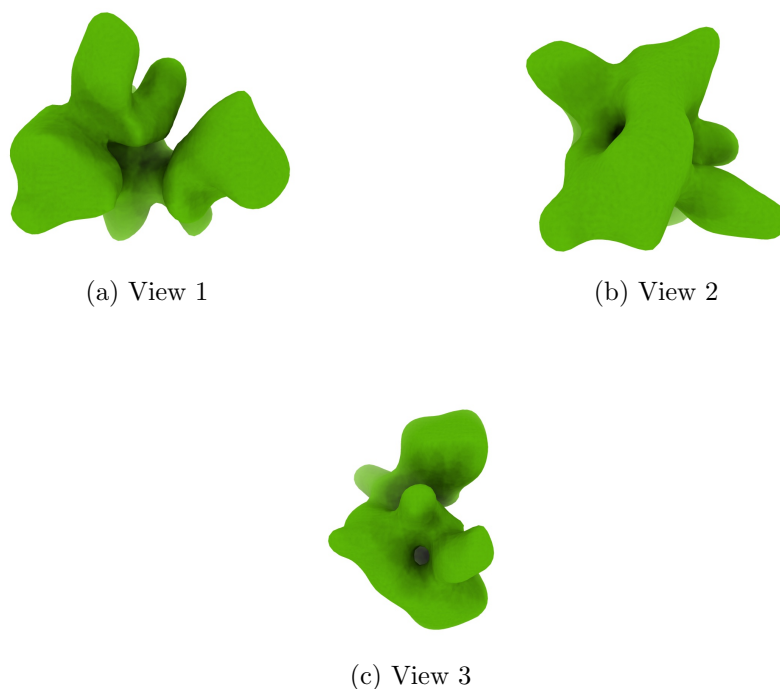
Figure 4: Isosurface at threshold=0.007400. Views generated by ChimeraX at a the following X, Y, Z angles: View 1 (0, -90, -90), View 2 (-90, 0, -90), View 3 (0, 0, 0).
