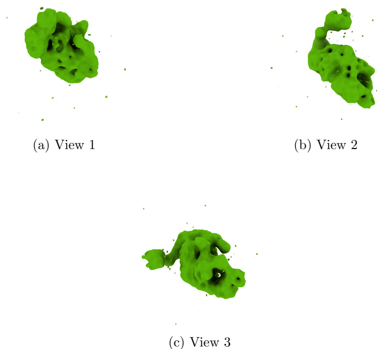
Figure 4: Isosurface at threshold=0.023400. Views generated by ChimeraX at a the following X, Y, Z angles: View 1 (0, -90, -90), View 2 (-90, 0, -90), View 3 (0, 0, 0).
