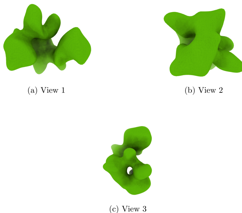
Figure 4: Isosurface at threshold=0.007010. Views generated by ChimeraX at a the following X, Y, Z angles: View 1 (0, -90, -90), View 2 (-90, 0, -90), View 3 (0, 0, 0).
