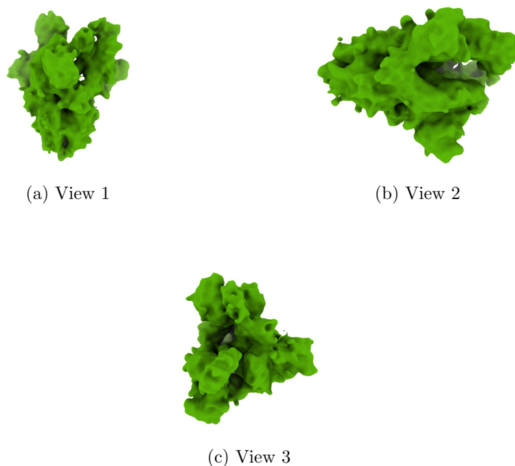
Figure 4: Isosurface at threshold=0.006870. Views generated by ChimeraX at a the following X, Y, Z angles: View 1 (0, -90, -90), View 2 (-90, 0, -90), View 3 (0, 0, 0).
