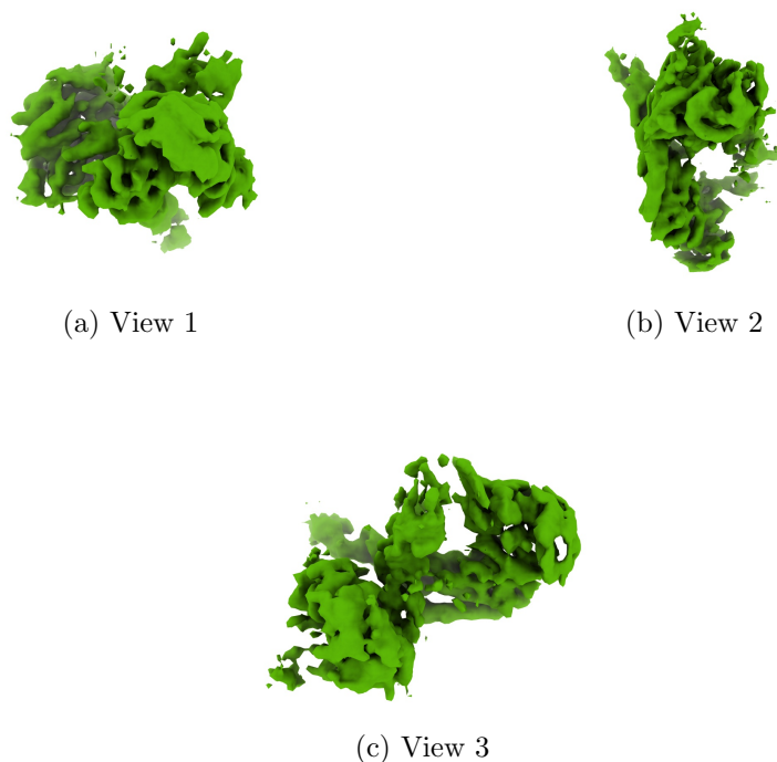
Figure 4: Isosurface at threshold=11.000000. Views generated by ChimeraX at a the following X, Y, Z angles: View 1 (0, -90, -90), View 2 (-90, 0, -90), View 3 (0, 0, 0).
